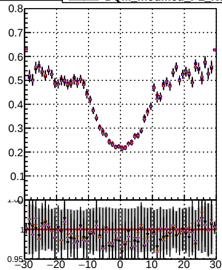
/data2/legianni/JSON-bkwd-fwd/no-modif/CMSSW_13_0_X_2023-01-24_1100/src/DQM_original Fake rate vs \nu
