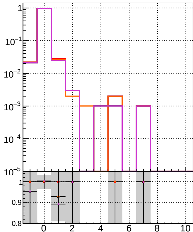
TruePVLocationIndexInRecoVertexCollection
