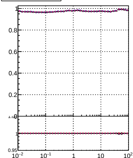
Fake rate vs v /data2/legianni/JSON-bkwd-fwd/no-modif/CMSSW_13_0_X_2023-01-24_1100/src/DQM_original DQM modified PL New2 DQM modified PL New2
