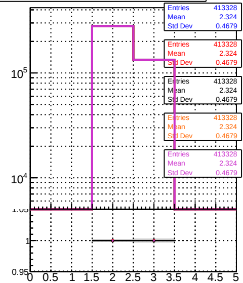
mean hit Legend: /data2/legami/JSON-bkwd-fwd/no-modif/CMSW_13_0_X_2023-01-24-1100/src/DQM_original (blue), DQM modified PL (red), DQM modified PL New1 (orange), DQM modified PL New2 (purple)
