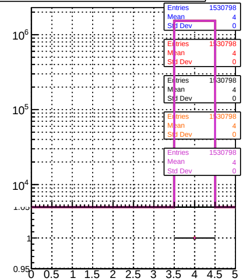
mean hit Legend: Data2/legami/JSON-bkwd-fwd/no-modif/CMSW_13_0_X_2023-01-24-1100/src/DQM_original DOM modified PL DOM modified PL New1 DOM modified PL New2
