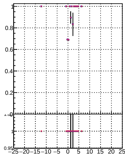
/data2/lojanni/JSON-bkwd-fwd/no-modif/CMSSW_13_0_X_2023-01-24-1100/src/DQM-original Fake rate vs d DQM-modified PL New2
