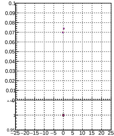
/data2/lojanni/JSON-bkwd-fwd/no-modif/CMSSW_13_0_X_2023-01-24-1100/src/DQM-original Fake rate vs d DQM-modified PL New2
