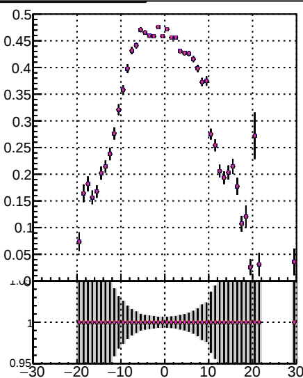
/data2/legiann/JSON-bkwd-fwd/no-modif/CMSSW_13_0_X_2023-01-24-1100/src/DQM-original Fake rate vs d
