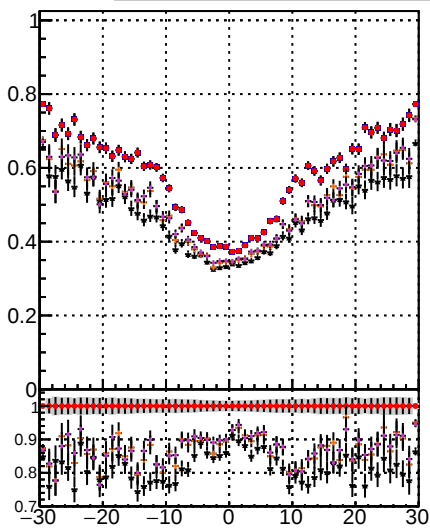
/data2/legion1/JSON-bkwd-fwd/no-modif/CMSSW_13_0_X_2023-01-24_1100/src/DQM_original Fake rate vs DQM modified PL New1 DQM modified PL New2
