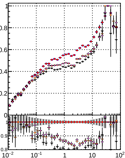
/data2/legion1/JSON-bkwd-fwd/no-modif/CMSSW_13_0_X_2023-01-24_1100/src/DQM_original Fake rate vs DQM modified PL New1 DQM modified PL New2
