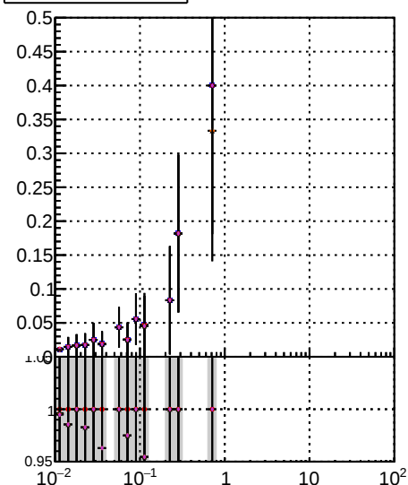
Fake rate vs v Legend: Blue line: /data2/legianni/JSON-bkwd-fwd/no-modif/CMSSW_13_0_X_2023-01-24_1100/src/DQM_original Red line: DQM-modified-PL-New1 Green line: DQM-modified-PL-New2 Black line: DQM-modified-PL-New3
