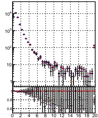
N of reco track vs. (data2/region1/JSON-blwd-fwd-no-modif/CMSSW_13_0_X_2023-01-24_1400/src/DQM-original)
