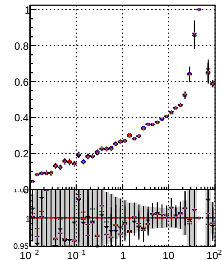
/data2/legianni/JSON-bkwd-fwd/no-modif/CMSSW_13_0_X_2023-01-24_1100/src/DQM_original Fake rate vs v... DQM modified PL New2 DQM modified PL New2
