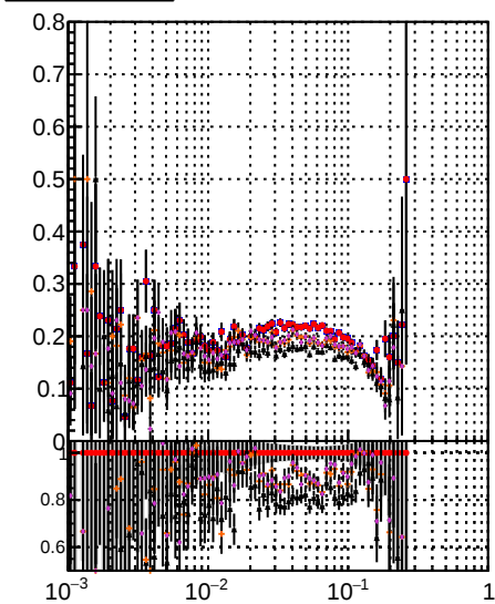
/data2/legionni/JSON-bkwd-fwd/no-modif/CMSSW_13_0_X-2023-01-24-1100/src/DQM_original Fake rate vs DQM modified PL DQM modified PL New1 DQM modified PL New2
