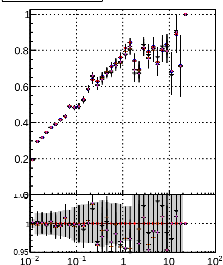
Fake rate vs v Legend: - \bullet /data2/legianni/JSON-bkwd-fwd/no-modif/CMSSW_13_0_X-2023-01-24-1100/src/DQM_original - \circ DQM-modified-PL - \times DQM-modified-PL-New1
