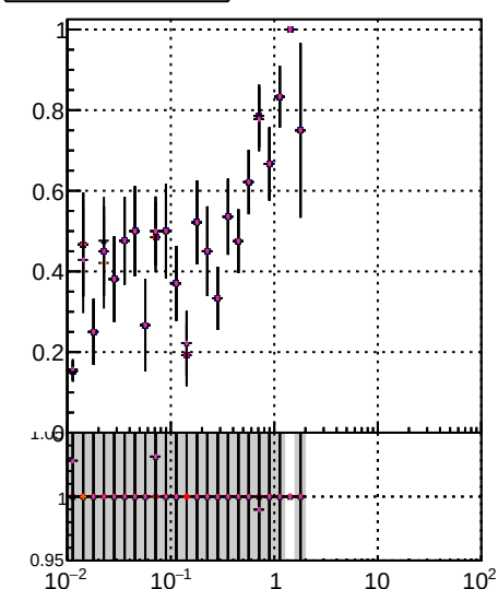
Fake rate vs v Legend: Blue line: DQM modified PL Red line: DQM modified PL New1 Green line: DQM modified PL New2 Black line: DQM modified PL
