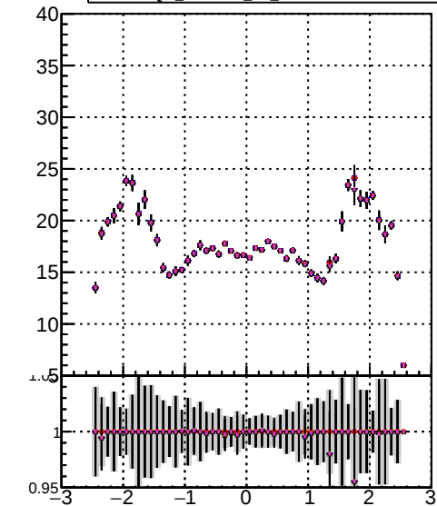
mean hit Legend: Data2/legion1, DOM modified PL, DOM modified PL New1, DOM modified PL New2, JSON-bkwd-fwd/no-modif, CMSSW_13_0_X_2023-01-24-1100/src/DQM_original
