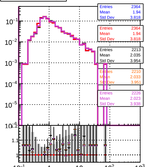
N of reco track vs pT
