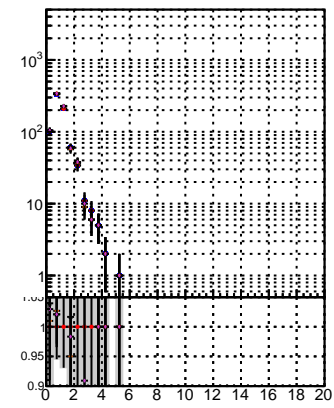
N of reco track vs. \chi^2 (data2/regions/JSON-blkwd-fwd-no-modif/GMSSW_13_0_X_2023-01-24_1400/src/DQM-original) BE-NEW1
