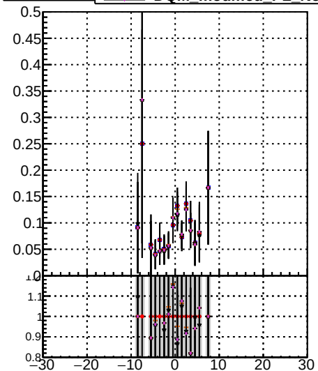
Fake rate vs v Legend: \bullet /data2/legianni/JSON-bkwd-fwd/no-modif/CMSSW_13_0_X_2023-01-24_1100/src/DQM_original \circ DQM modified PL \times DQM modified PL New1 \star DQM modified PL New2
