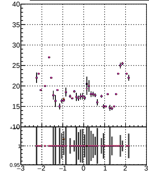
mean hit Legend: Data2/legam1, JSON-bkwd-fwd/no-modif, CMSSW_13_0_X_2023-01-24_1100/src/DQM_original, DQM modified PL, DQM modified PL New1, DQM modified PL New2
