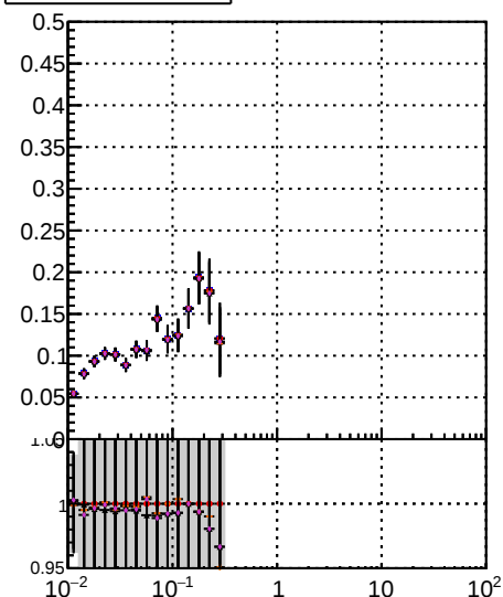
Fake rate vs v Legend: Blue line: /data2/legionni/JSON-bkwd-fwd/no-modif/CMSSW_13_0_X_2023-01-24_1100/src/DQM_original Red line: DQM modified PL Green line: DQM modified PL New1
