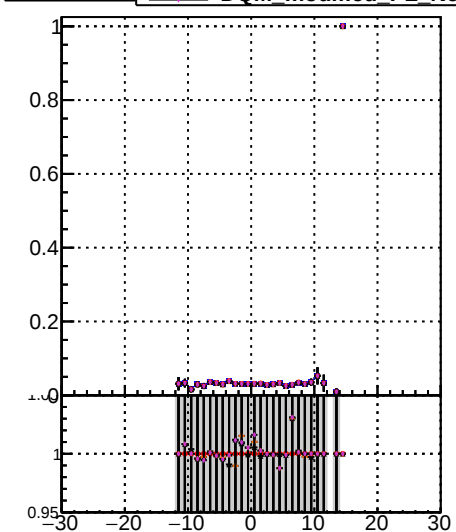
Fake rate vs v Legend: Blue line: /data2/legianni/JSON-bkwd-fwd/no-modif/CMSSW_13_0_X_2023-01-24_1100/src/DQM_original Red line: DQM-modified-PL-New1 Green line: DQM-modified-PL-New2
