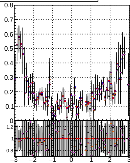
Pileup rate vs \phi
