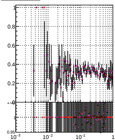
Fake rate vs /data2/legianni/JSON-bkwd-fwd/no-modif/CMSSW_13_0_X-2023-01-24-1100/src/DQM_original /data2/legianni/JSON-bkwd-fwd/no-modif/CMSSW_13_0_X-2023-01-24-1100/src/DQM_modified_PL-New1 /data2/legianni/JSON-bkwd-fwd/no-modif/CMSSW_13_0_X-2023-01-24-1100/src/DQM_modified_PL-New2
