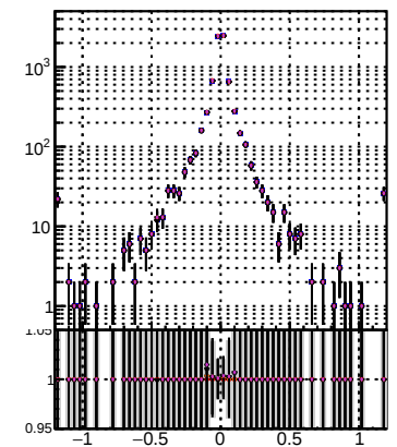
N of simulated tracks vs dz(PV) with zoomed-in x-axis
