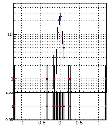
N of associated tracks (simToReco) vs dz(PV) with zoomed-in x-axis
