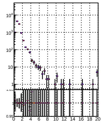
N of reco track vs. \chi^2 (data2/region0/JSON-blwd-fwd/no-mod/CMSW_13_0_X_2023-01-24_1100/src/DQM-original)
