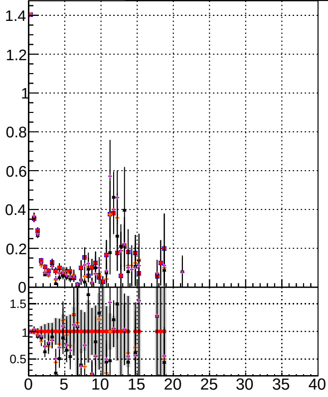
K_S^0 tracking fake rate Legend: \blacksquare /data2/legianni/JSON-bkwd-fwd/no-modif/CMSSW_13_0_X_2023-01-24-1100/src/DQM_original \bullet DQM_modified \blacktriangle DQM_modified PL \blacklozenge DQM_modified PL New1 \blacktriangledown DQM_modified PL New2
