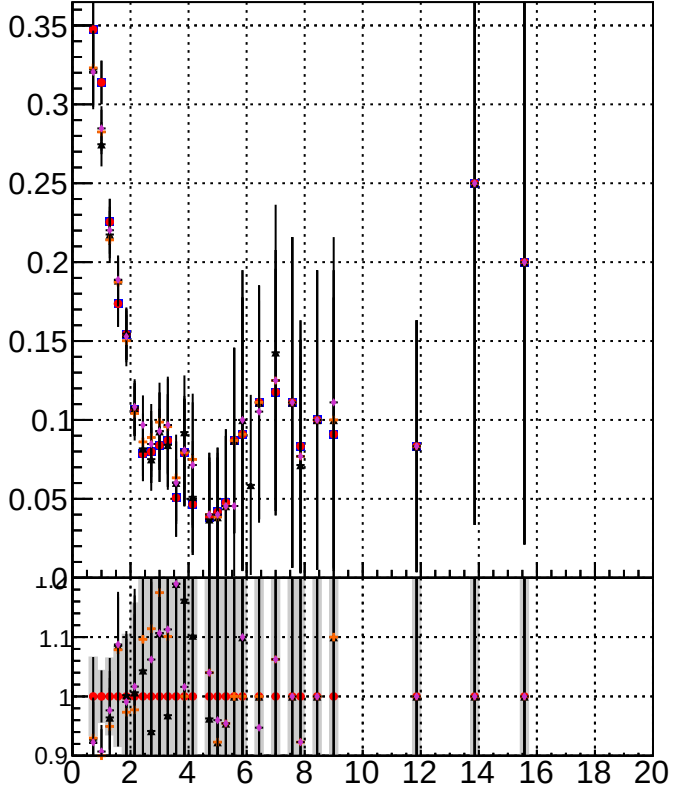
K_S^0 tracking fake rate vs p_T
