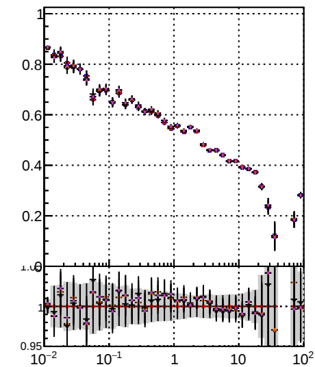
/data2/legion1/JSON-bkwd-fwd/no-modif/CMSSW_13_0_X_2023-01-24_1100/src/DQM_original Fake rate vs v DQM modified PL New2 DQM modified PL New1
