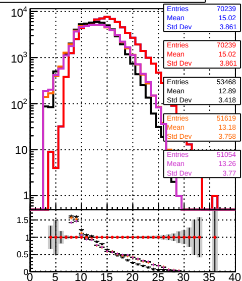
mean hit data2legion DOM modified JSON-bkwd-fwd/no-modif CMSSW_13_0_X_2023-01-24_1100/src/DQM_original DOM modified PL DOM modified PL New1 DOM modified PL New2
