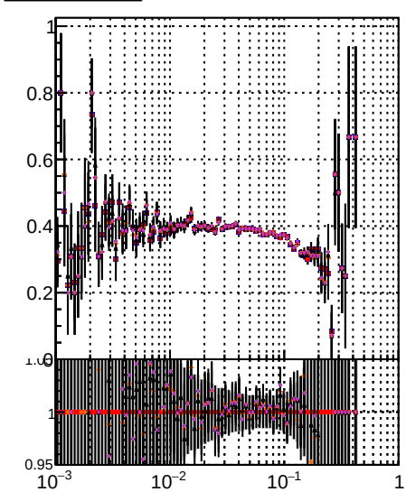
Fake rate vs /data2/legion/json-bkwd-fwd/no-modif/CMSSW_13_0_X_2023-01-24_1100/src/DQM_original DQM modified PL New1 DQM modified PL New2
