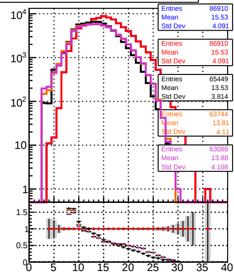
data2legami JSON-bkwd-fwd/no-modif/CMSW_13_0_X_2023-01-24-1100/src/DQM_original DQM modified PL DQM modified PL New1 DQM modified PL New2
