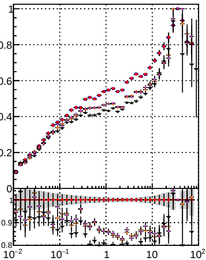
Fake rate vs DQM modified PL New1 DQM modified PL New2
