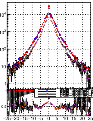
N of reco track vs dxy
