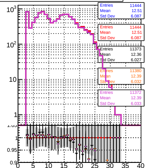
mean hit data2/legami/JSON-bkwd-fwd/no-modif/CMSW_13_0_X_2023-01-24_1100/src/DQM_original DOM modified PL New1 DOM modified PL New2
