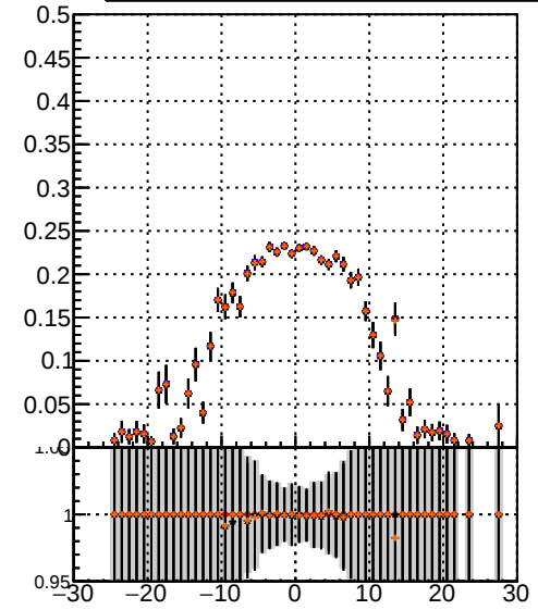
Efficiency vs vertpos Legend: — data2/legianni/JSON-bkwd-fwd/no-modif/CMSSW_13_0_X_2023-01-24-1100/src/DQM_original — DQM_modified — DQM_modified_PL — DQM_modified_PL_New1
