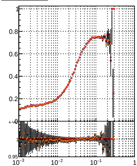
Fake rate vs dr DQM modified PL New1
