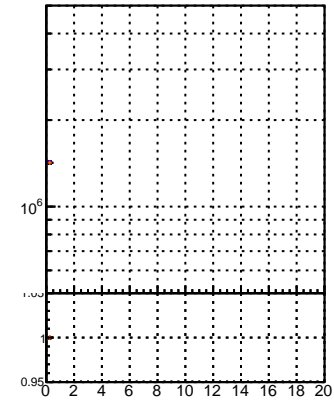
N of reco track vs. \chi^2 (data2/legions/JSON blwd fwd/no modif/CMSW_13_0_X_2023_01_24_1400/src/DQM_original)
