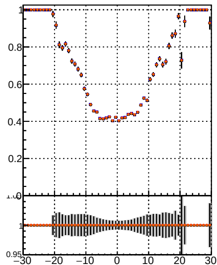
Legend: - Blue line: /data2/legion/JSON-bkwd-fwd/no-modif/CMSSW_13_0_X_2023-01-24-1100/src/DQM-original - Black line: DQM-modified - Orange line: DQM-modified PL New1
