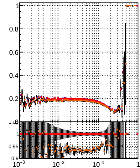
Fake rate vs dr Legend: - data2/legianni/JSON-bkwd-fwd/no-modif/CMSSW_13_0_X_2023-01-24-1100/src/DQM_original - DQM modified PL New1
