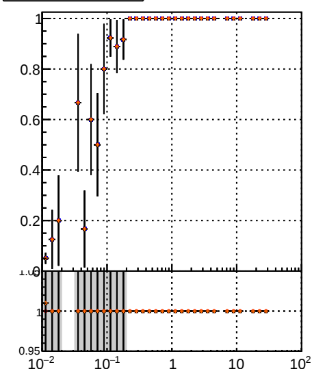
Fake rate vs v data2/legianni/JSON-bkwd-fwd/no-modif/CMSSW_13_0_X_2023-01-24-1100/src/DQM_original DQM modified PL New1
