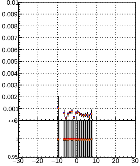
/data2/legion1/JSON-bkwd-fwd/no-modif/CMSSW_13_0_X_2023-01-24-1100/src/DQM-original Fake rate vs d Legend: Blue line: DQM modified PL New1 Red line: DQM modified PL New1 Orange line: DQM modified PL New1
