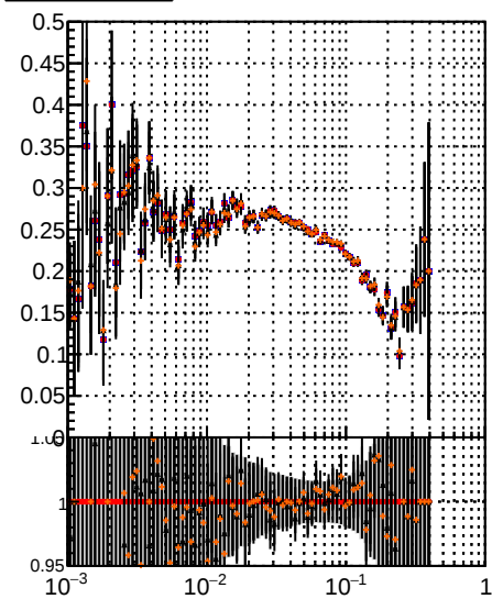
Fake rate vs dr Legend: - data2/legianni/JSON-bkwd-fwd/no-modif/CMSSW_13_0_X_2023-01-24-1100/src/DQM_original - DQM modified PL New1 - DQM modified PL
