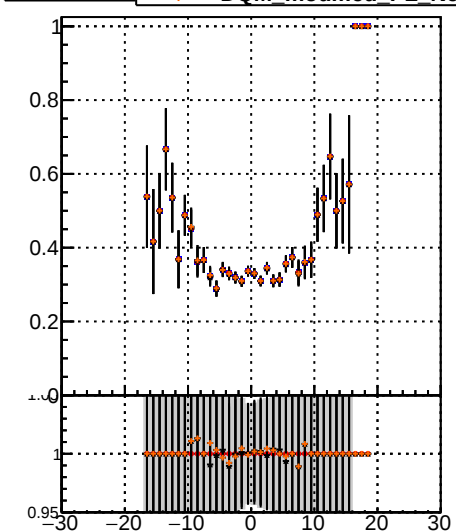
Fake rate vs v data2/legianni/JSON-bkwd-fwd/no-modif/CMSSW_13_0_X_2023-01-24-1100/src/DQM_original BQM modified PL BQM modified PL New1
