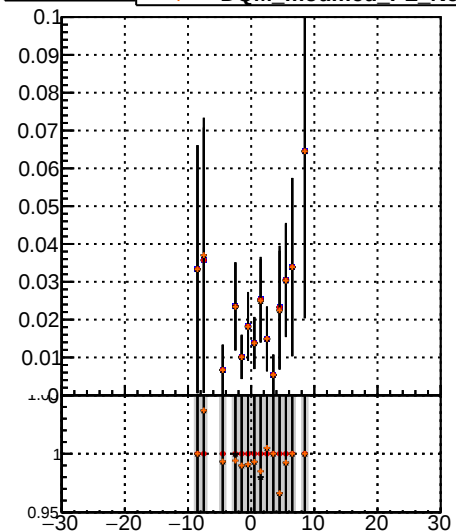
Fake rate vs verpos Legend: - data2/legianni/JSON-bkwd-fwd/no-modif/CMSSW_13_0_X_2023-01-24-1100/src/DQM_original - DQM modified PL New1 - DQM modified PL - DQM modified PL
