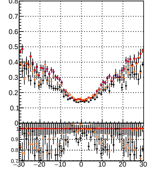
— /data2/legianni/JSON-bkwd-fwd/no-modif/CMSW_13_0_X_2023-01-24-1100/src/DQM_original ● DQM_modified ● DQM_modified_PL ● DQM_modified_PL_New1 Efficiency vs. sim PV z
