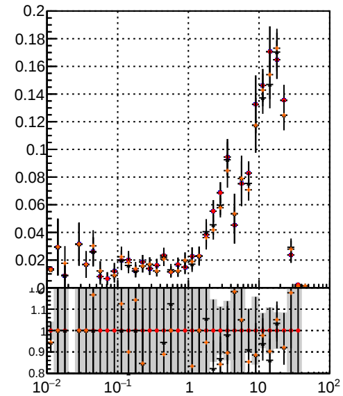
— /data2/legianni/JSON-bkwd-fwd/no-modif/CMSW_13_0_X_2023-01-24-1100/src/DQM_original ● DQM_modified ● DQM_modified_PL ● DQM_modified_PL_New1 Efficiency vs. sim PV z
