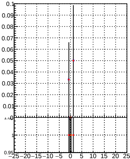
/data2/legion/JSON-bkwd-fwd/no-modif/CMSSW_13_0_X_2023-01-24-1100/src/DQM_original Fake rate vs d DQM modified DQM modified PL New1
