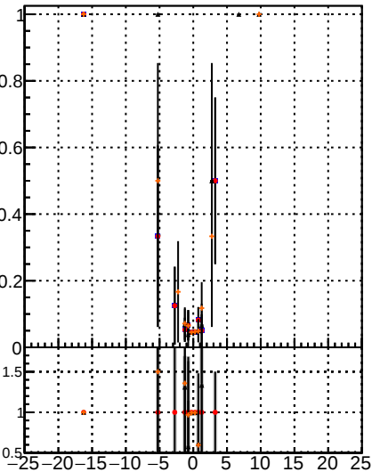
/data2/legion/JSON-bkwd-fwd/no-modif/CMSSW_13_0_X_2023-01-24-1100/src/DQM_original Fake rate vs d DQM modified DQM modified PL New1
