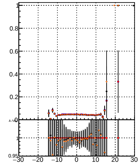
/data2/legion/JSON-bkwd-fwd/no-modif/CMSSW_13_0_X_2023-01-24-1100/src/DQM_original Fake rate vs d DQM modified DQM modified PL New1
