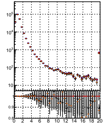
N of reco track vs. \chi^2 for data2/legion/JSON blwd fwd/no mod/GMSSW_13_0_X_2023 01 24 1400/src/DQM_original
