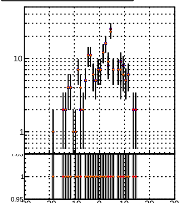
N of associated (recoToSim) loopier tracks vs transverse ref point position
