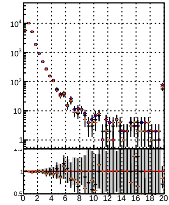
data2/legion1/JSON/blwd-fwd/no-mod/GMSSW_13_0_X_2023-01-24_1100/src/BQM_original N of reco track vs. \chi^2 BQM modified BL New1
