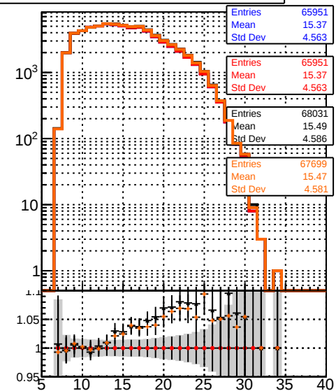
mean hit Legend: /data2/legianni/JSON-bkwd-fwd/no-modif/CMSW_13_0_X_2023-01-24-1100/src/DQM_original (blue line), DQM_modified (red line), DQM_modified_PL (black line), DQM_modified_PL_New1 (orange line)
