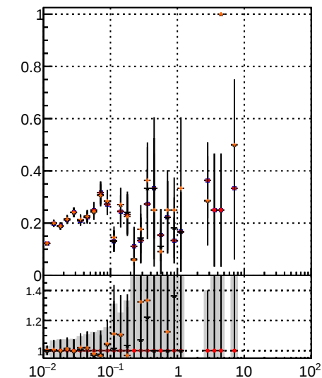
data2/legianni/JSON-bkwd-fwd/no-modif/CMSSW_13_0_X_2023-01-24-1100/src/DQM_original Fake rate vs verpos DQM modified PL New1
